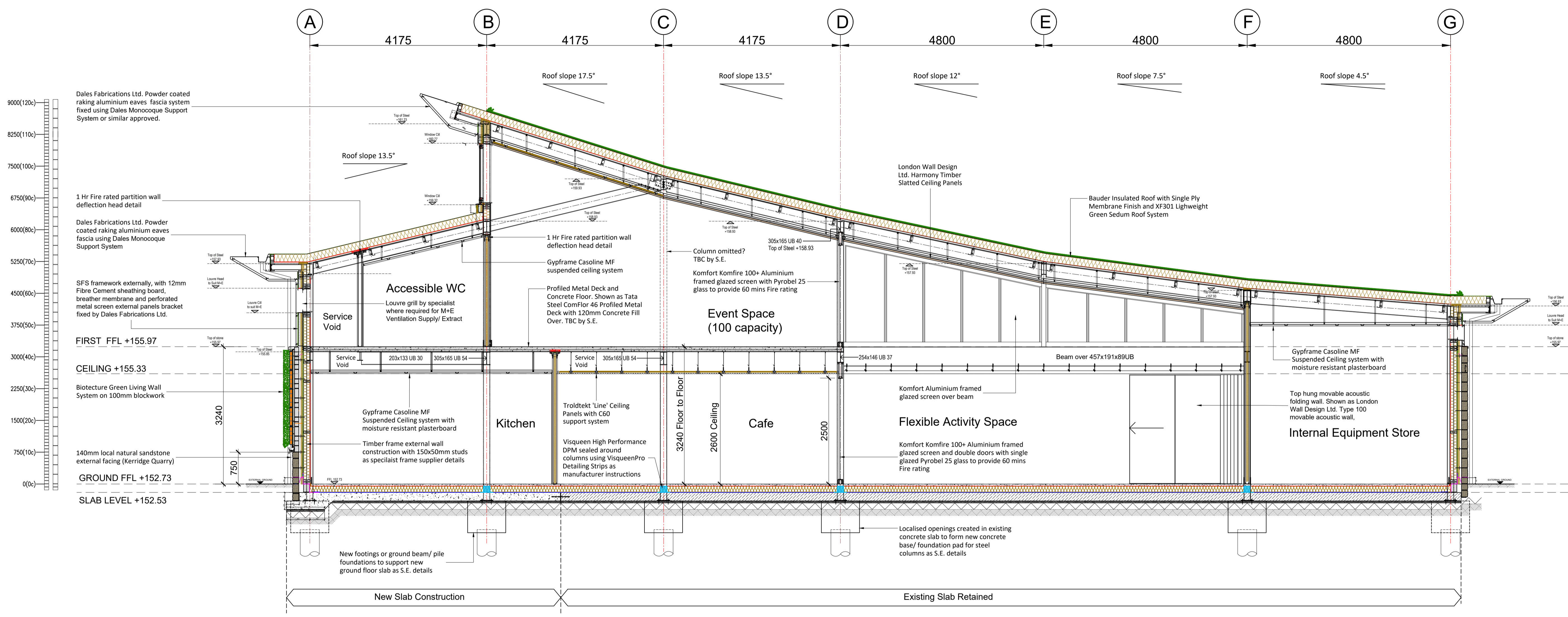
SECTION AA (Grid Line 03)
