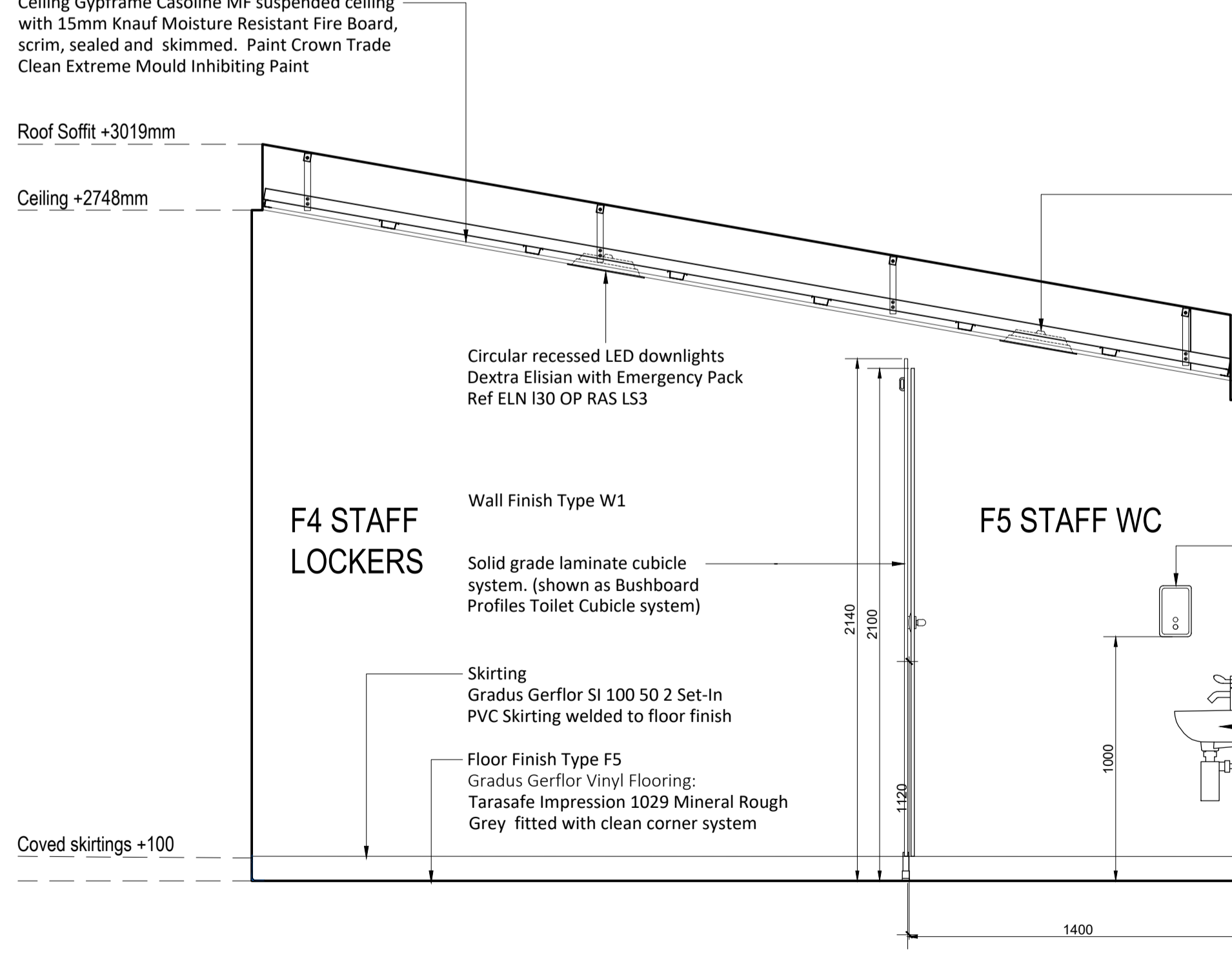
ELEVATION C
